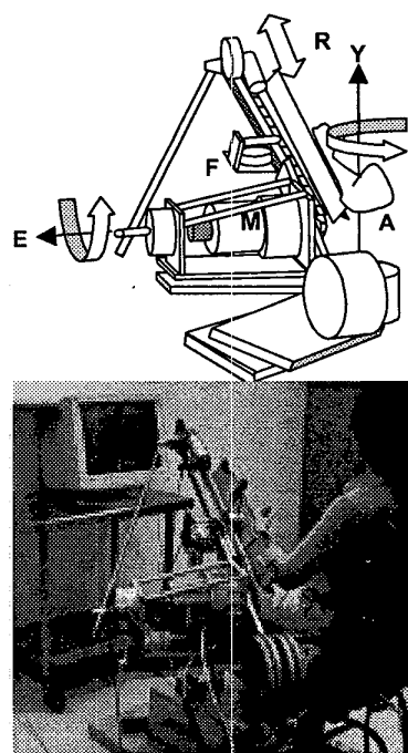
Fig. 1. Diagram and photo of the ARM Guide
